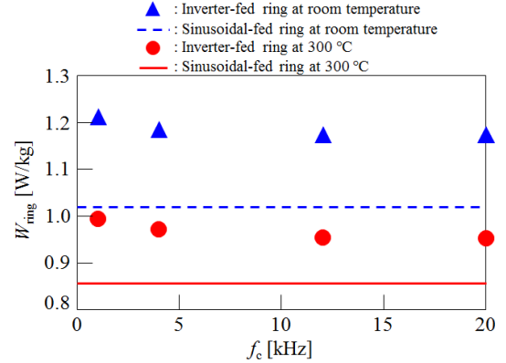
Fig. 5. Experimentally obtained iron losses of ring specimen as a function of carrier frequency at f_0 = 50 Hz and B = 1 T. Tests are performed at carrier frequencies f_c of 1, 4, 12, and 20 kHz. The iron losses is calculated by integrating H and B with Eq. (3)
